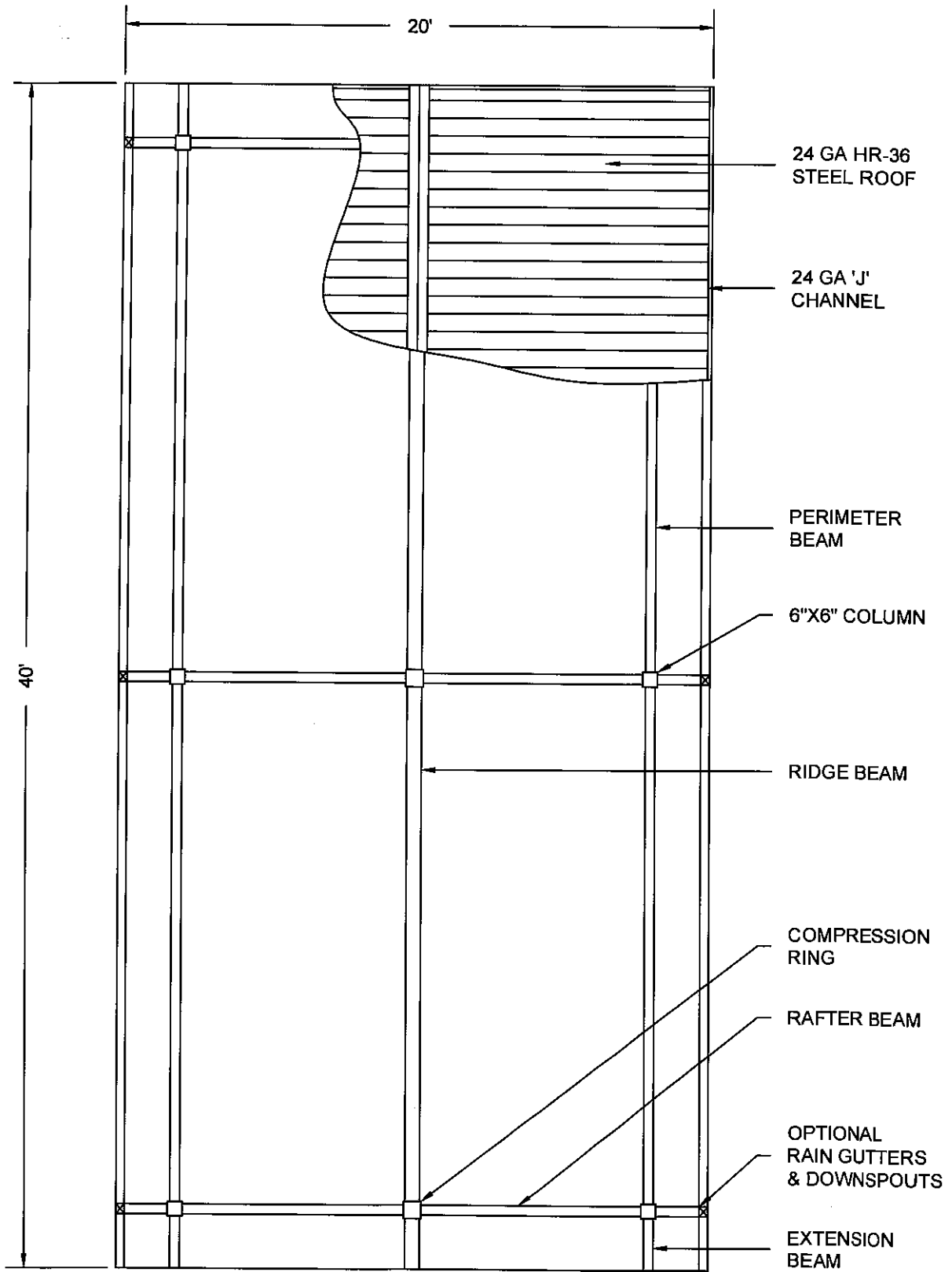
PLAN VIEW 20'X40'
